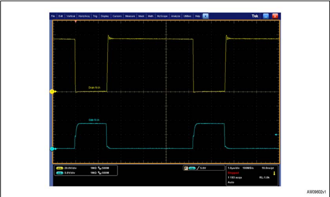
Figure 19. Primary side power MOSFET waveforms at 0 A load
