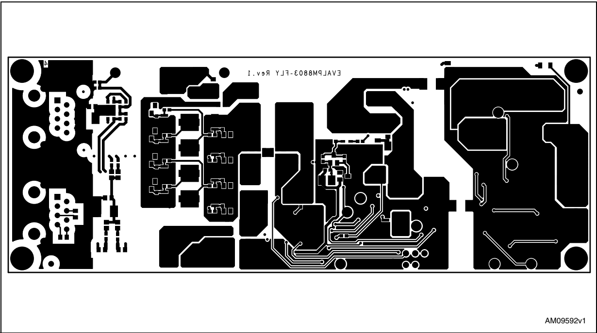
Figure 9. Bottom layer
