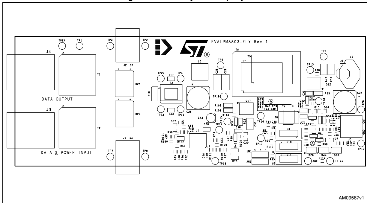
Figure 4. Assembly view: top layer
