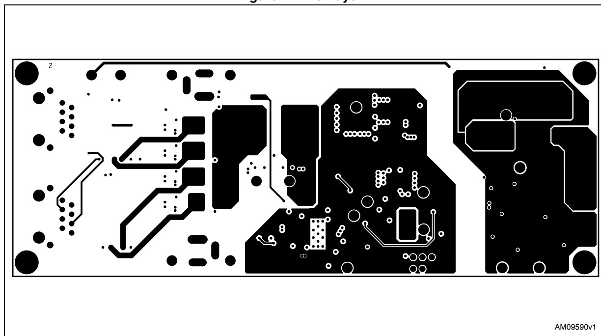
Figure 7. Inner layer 1
