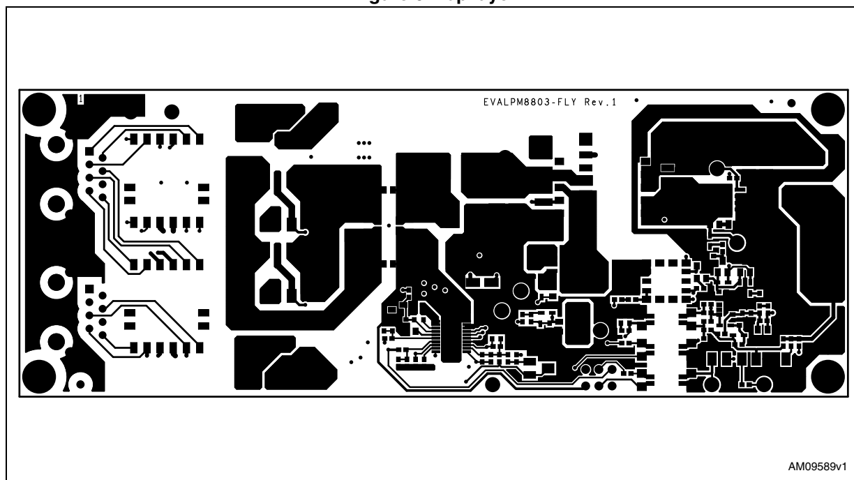
Figure 7. Inner layer 1
