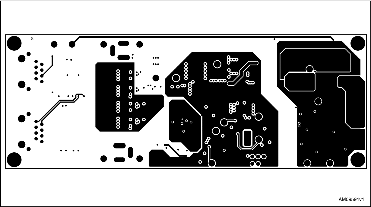
Figure 8. Inner layer 2
