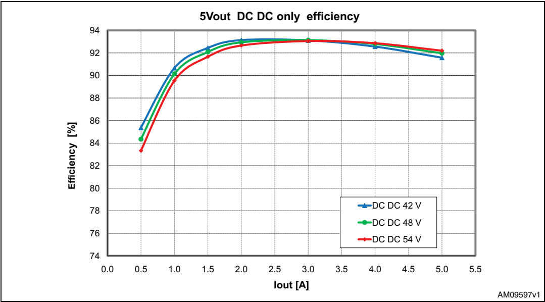
Figure 14. DC-DC only efficiency measurements
